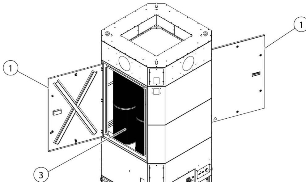
Fig. 27: Changing filters
