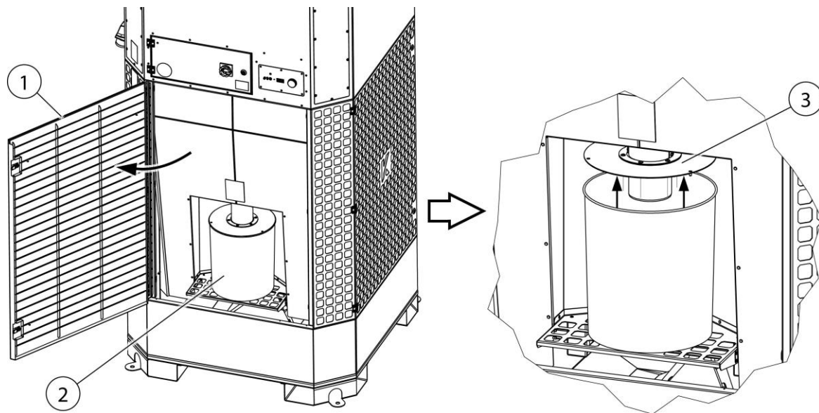
Fig. 23: Changing the dust collection container
