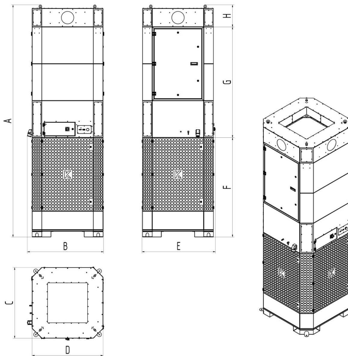
Fig. 33: Dimensions sheet
