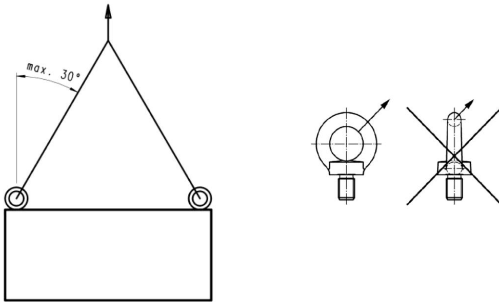
Fig. 4: Information on lifting procedure
