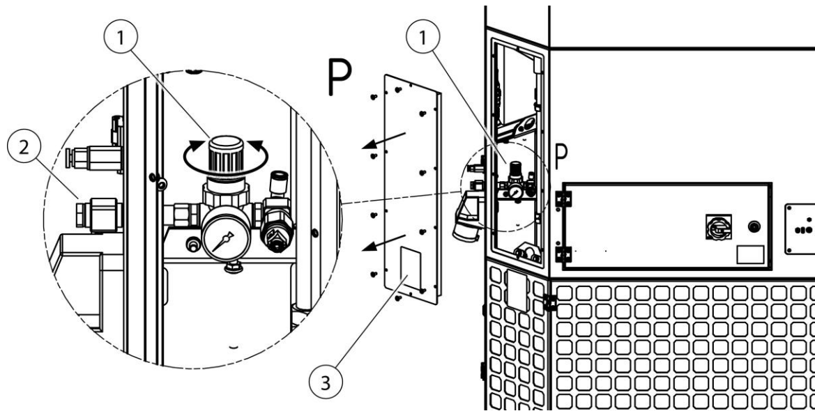
Fig. 26: Setting the compressed air regulator
