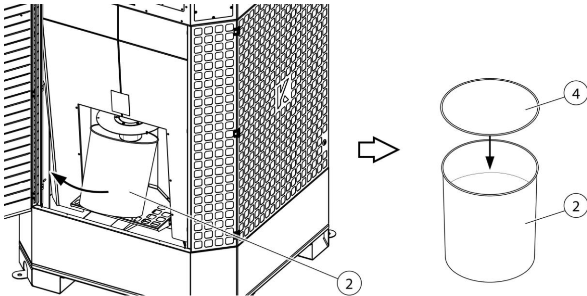
Fig. 24: Changing the dust collection container
