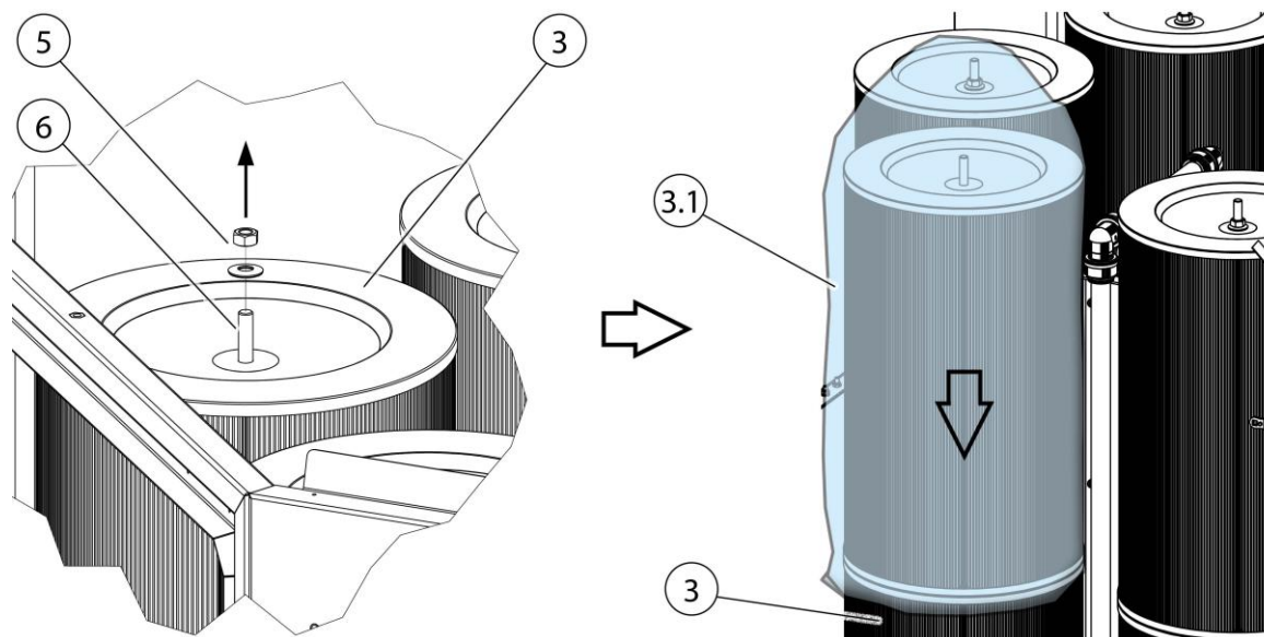
Fig. 28: Changing filters – Removing the filter
