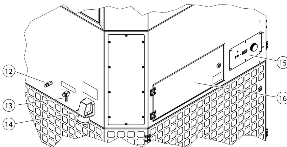
Fig. 3: Product description
