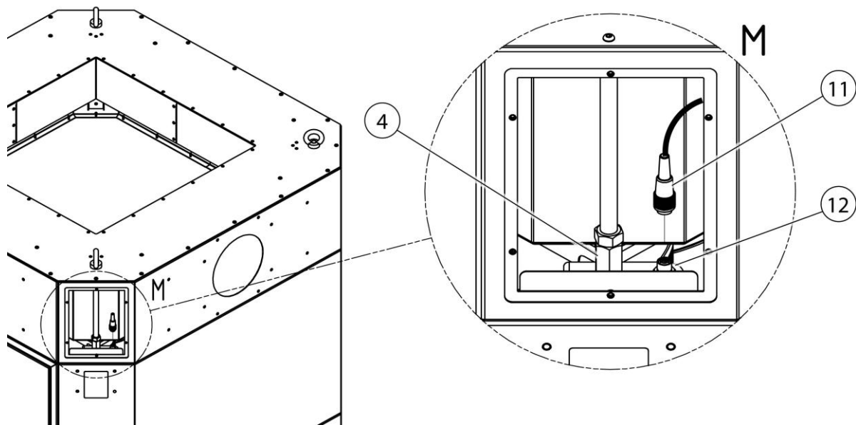
Fig. 18: Assembly – Intake unit with filter component
